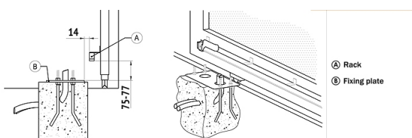
PREDISPOSITION FOR STANDARD INSTALLATION
