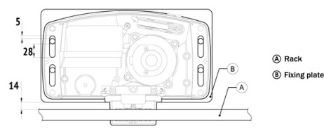
PREDISPOSITION FOR STANDARD INSTALLATION
